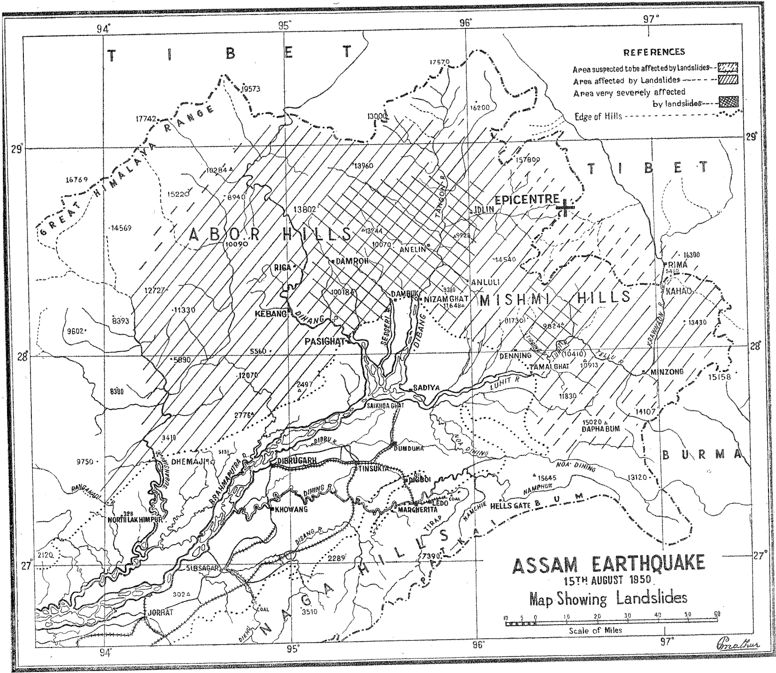
ASSAM EARTHQUAKE, 15th AUGUST, 1950—MAP SHOWING LANDSLIDES.
